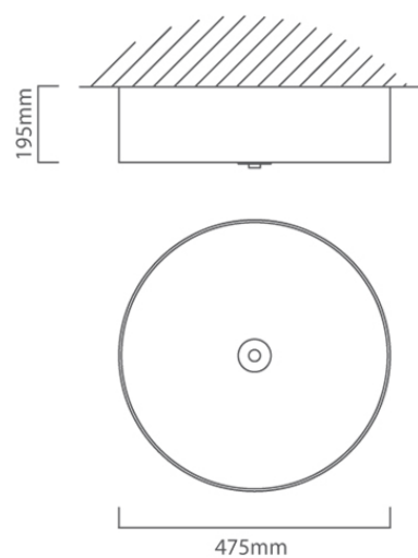
C122 CAD DIAGRAM
