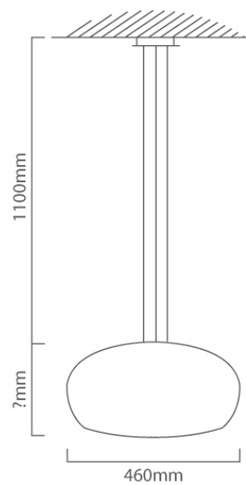
P158 CAD DIAGRAM
