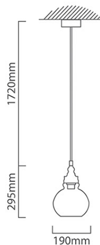
P589 CAD DIAGRAM
