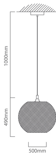
P770 CAD DIAGRAM
