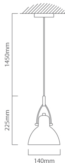
P904B CAD DIAGRAM
