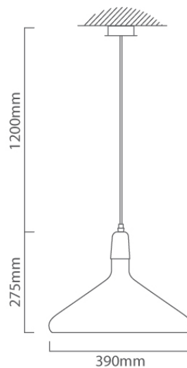
P944 CAD DIAGRAM
