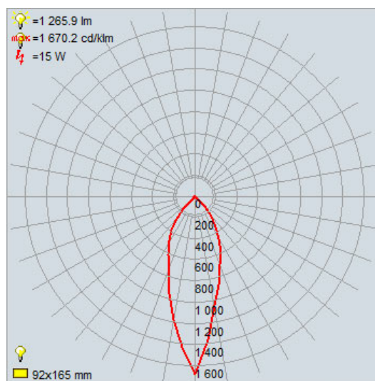
PR346 IES DIAGRAM
