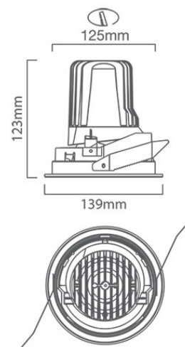
PR377 CAD DIAGRAM
