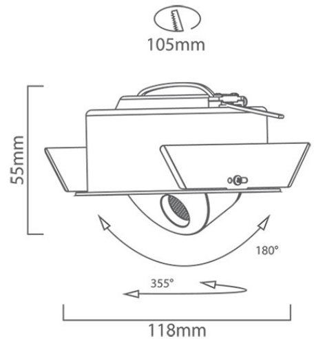
PR380 CAD DIAGRAM
