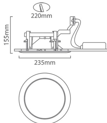
PR407 CAD DIAGRAM
