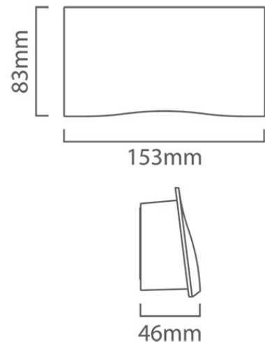
PR411 CAD DIAGRAM
