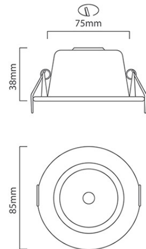
PR459 CAD DIAGRAM
